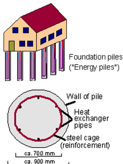
Figure 12. Energy piles and cross-section of a pile with three loops.
